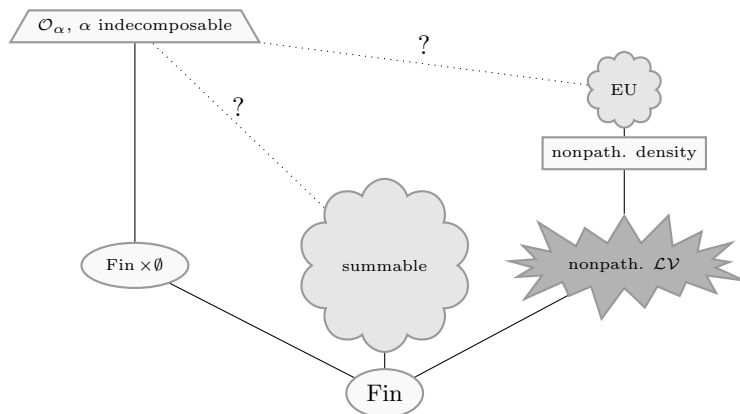
FIGURE 0.0.6. Embeddability of quotients assuming OCA_T and MA(\sigma\text{-linked}) . Relations along the dotted lines are not known to be refuted by any forcing axioms, but they do not exist in models constructed in [60] and [75].
